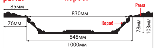
КР100-6 (1000x1000x103)
