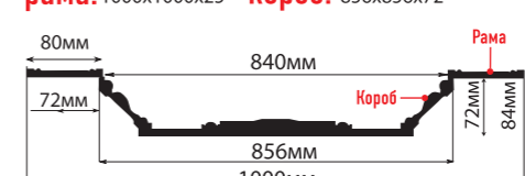
KP100-933 (1000x1000x84)
