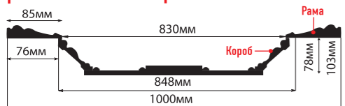
KP100-7D (1000x1000x103) рама: 1000x1000x25 короб: 848x848x78
