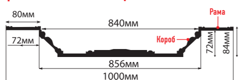
KP100-553 (1000x1000x84)
